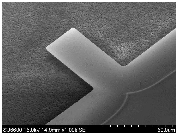
Si Cantilever Processed with Metal-Induced Lateral Crystallization
