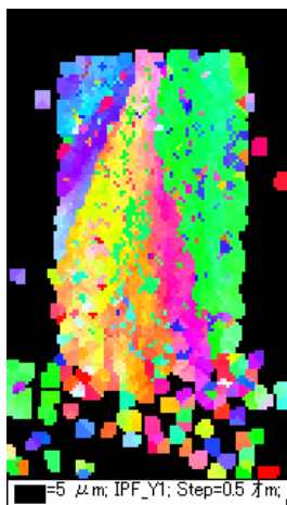
Si Cantilever Processed with Metal-Induced Lateral Crystallization
