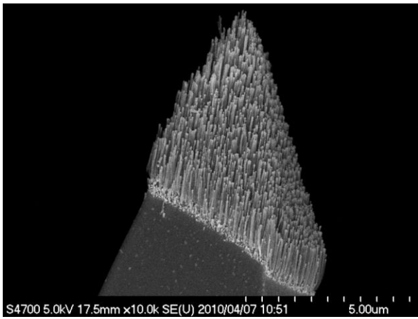
Carbon Nanotubes on AFM tip
