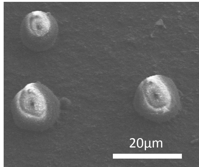
Local Plasma Irradiation on Polyethylene Particles
